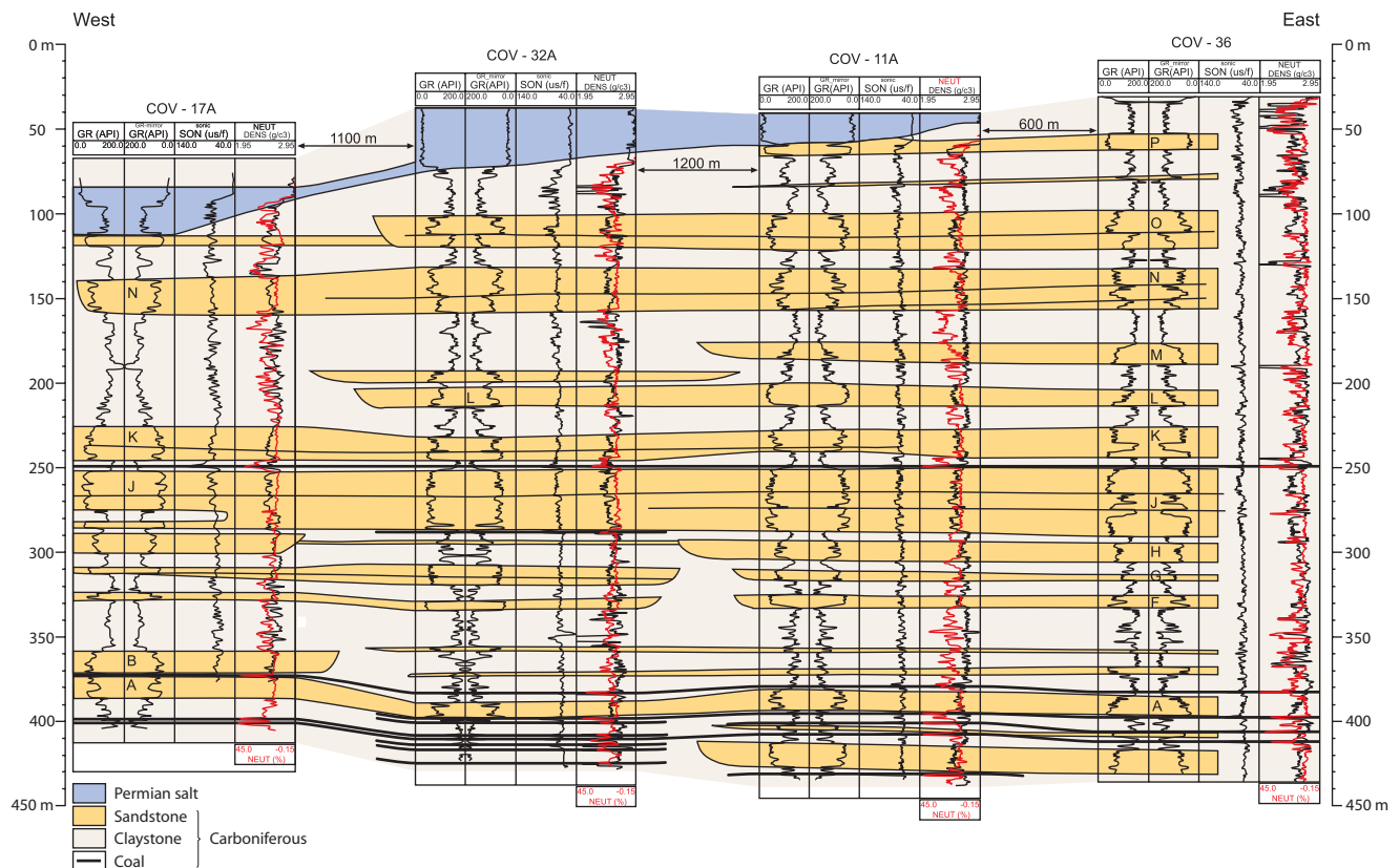
Fig. 7. Well log panel showing interpretation (for location of this panel see Fig. 1).
