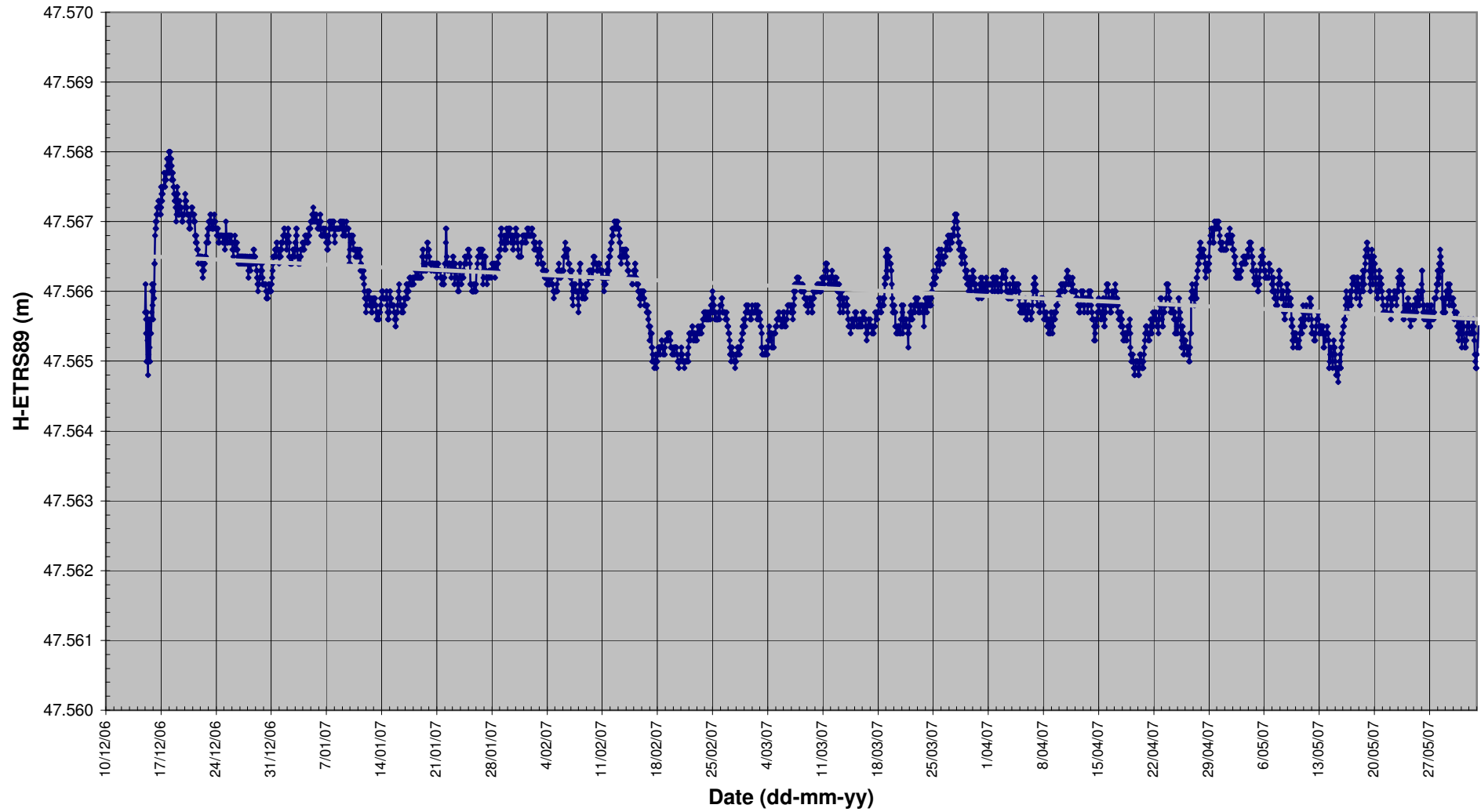
GEO++ H-ETRS89 MODD mm/HOUR PE 15 dec 2006 - 2 june 2007 + trend least squares method
