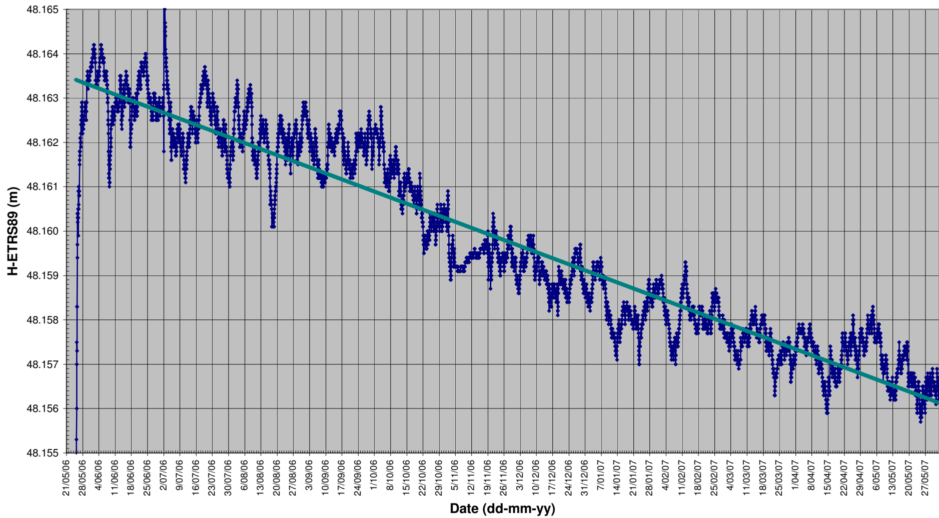
GEO++ H-ETRS89 AME1 mm/HOUR PE 25 may 2006 - 2 june 2007 + trend least squares method
