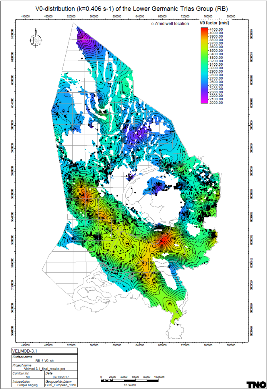
Figure 52 V_0 distribution of the Lower Germanic Trias Group
