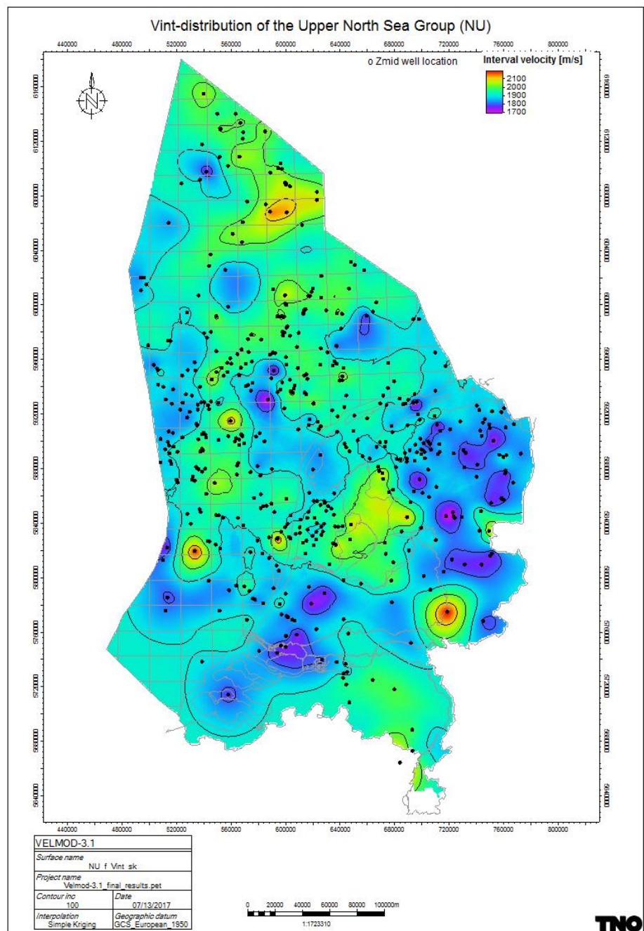
Figure 27 V_{int} distribution of the Upper North Sea Group
