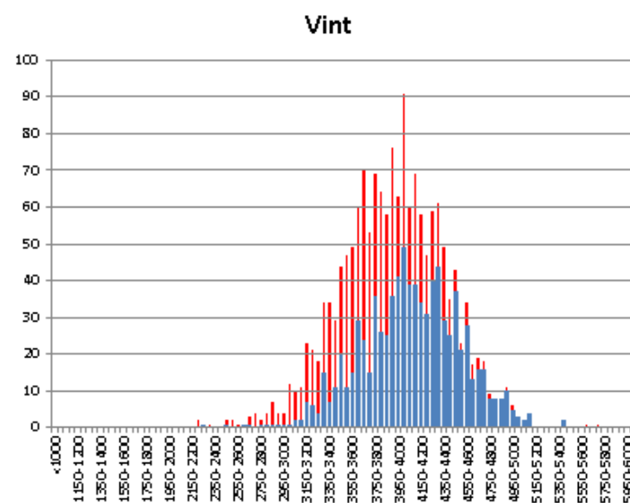
Figure 63 Interval velocity distribution of basins (blue) compared to the total distribution (red).
