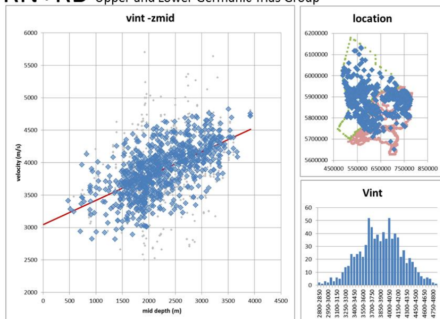
Figure 13 Interval velocity vs mid-depth (left; grey points are discarded from regression analysis), distribution (lower right) and location (upper right) of interval velocities of the Upper and Lower Germanic Trias groups.
