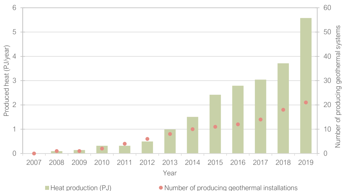
Figure 5.5 Annual production of geothermal energy (PJ/year).
