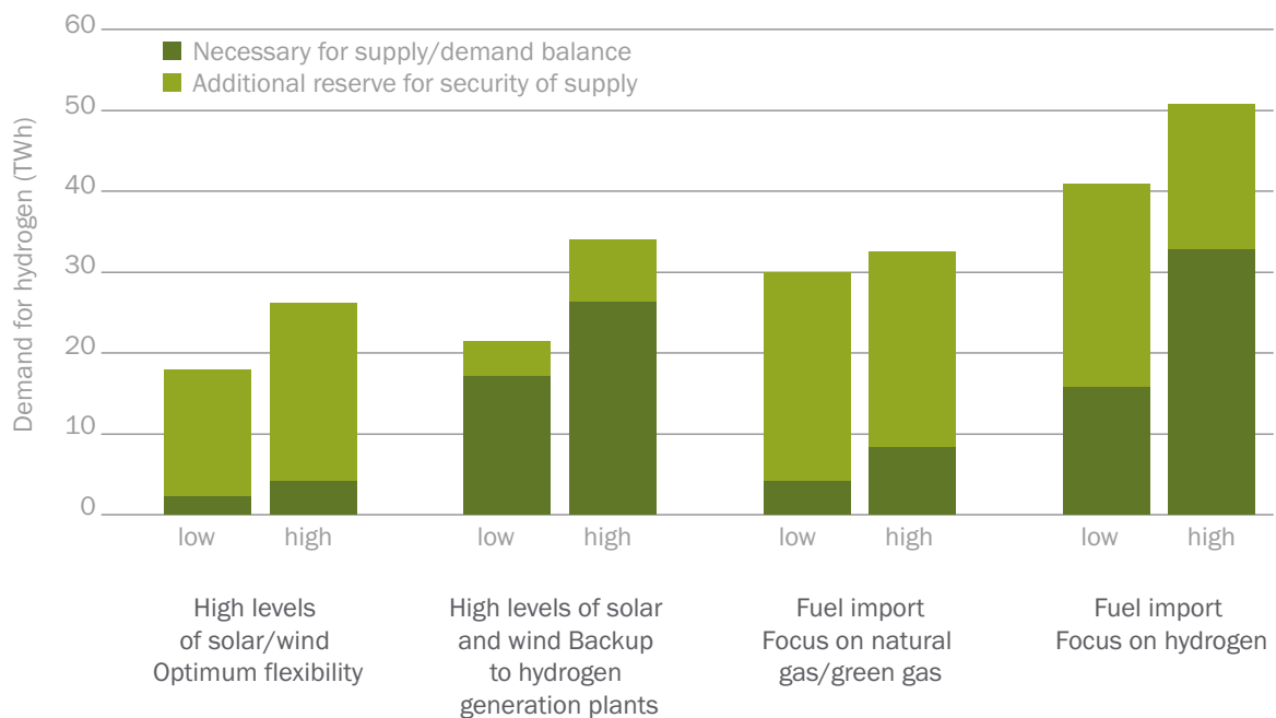
Figure 4: Potential demand for hydrogen storage in 2050 in relation to various developments in the energy system.
