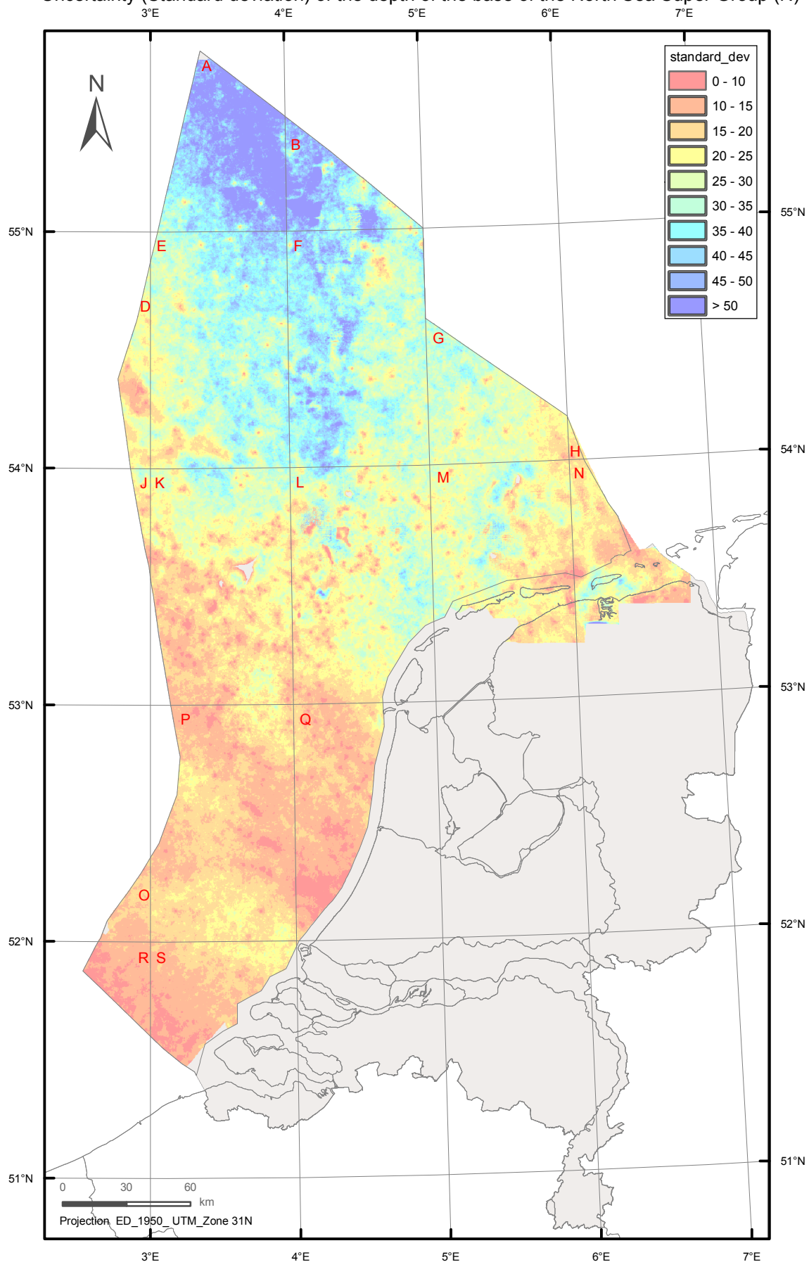
Uncertainty (Standard deviation) of the depth of the base of the North Sea Super Group (N)
