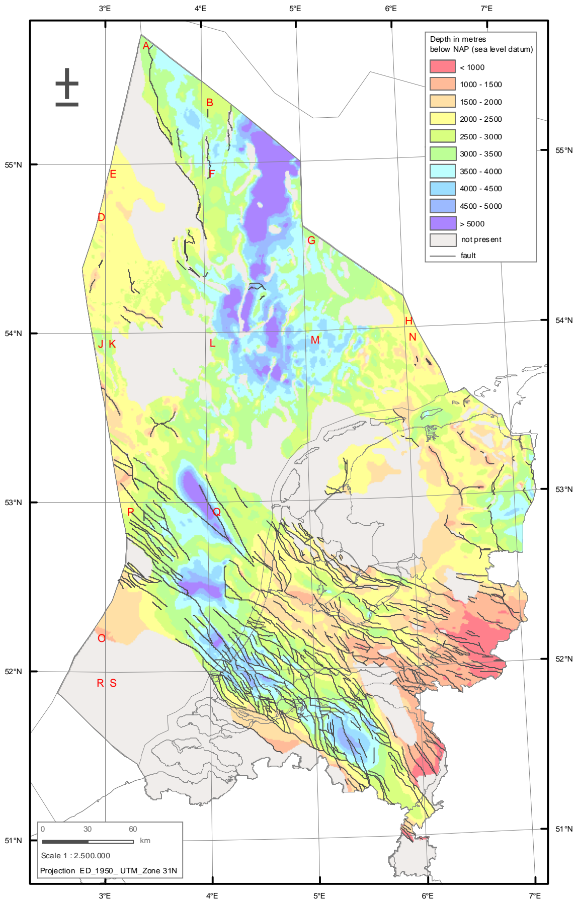
Fig 6a Depth of the base of the Lower Germanic Trias Group RB
