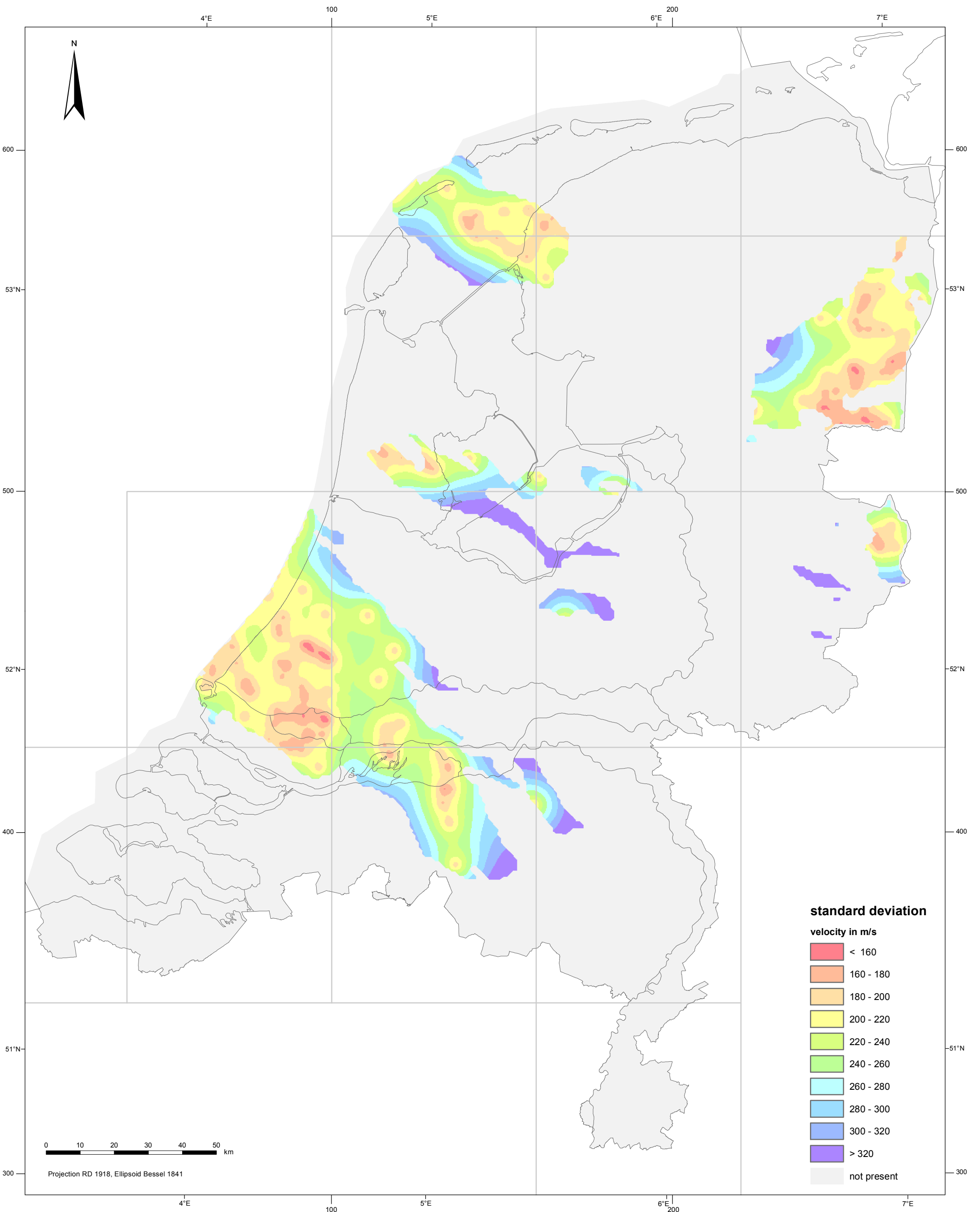
Uncertainty (standard deviation) of the velocity of the Schieland and Niedersachsen Groups (S)
