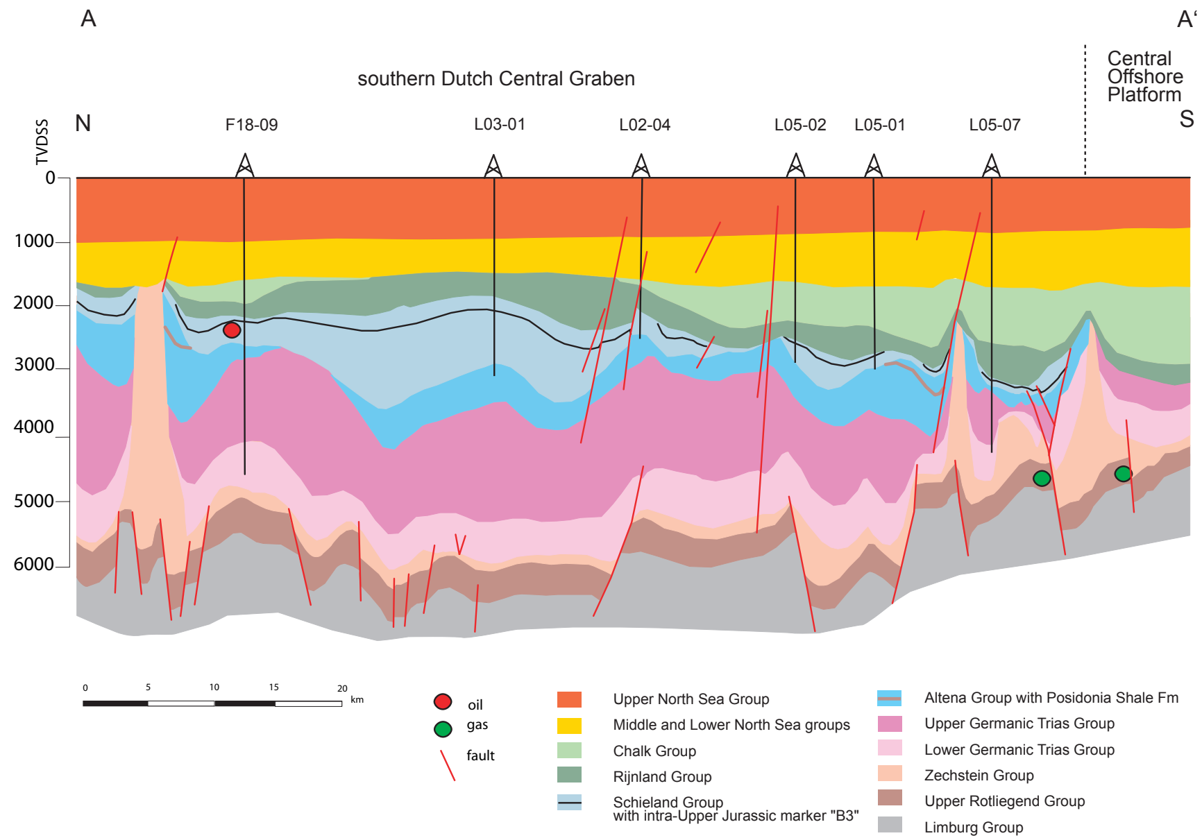
Cross section A-A' This geological profile runs N-S through the southern part of the Dutch Central Graben where both Lower and Upper Jurassic deposits are present. Both oil and gas fields are found in this area. Major faulting occurred in the area of the Hantum Boundary Fault from Carboniferous until Tertiary age.
