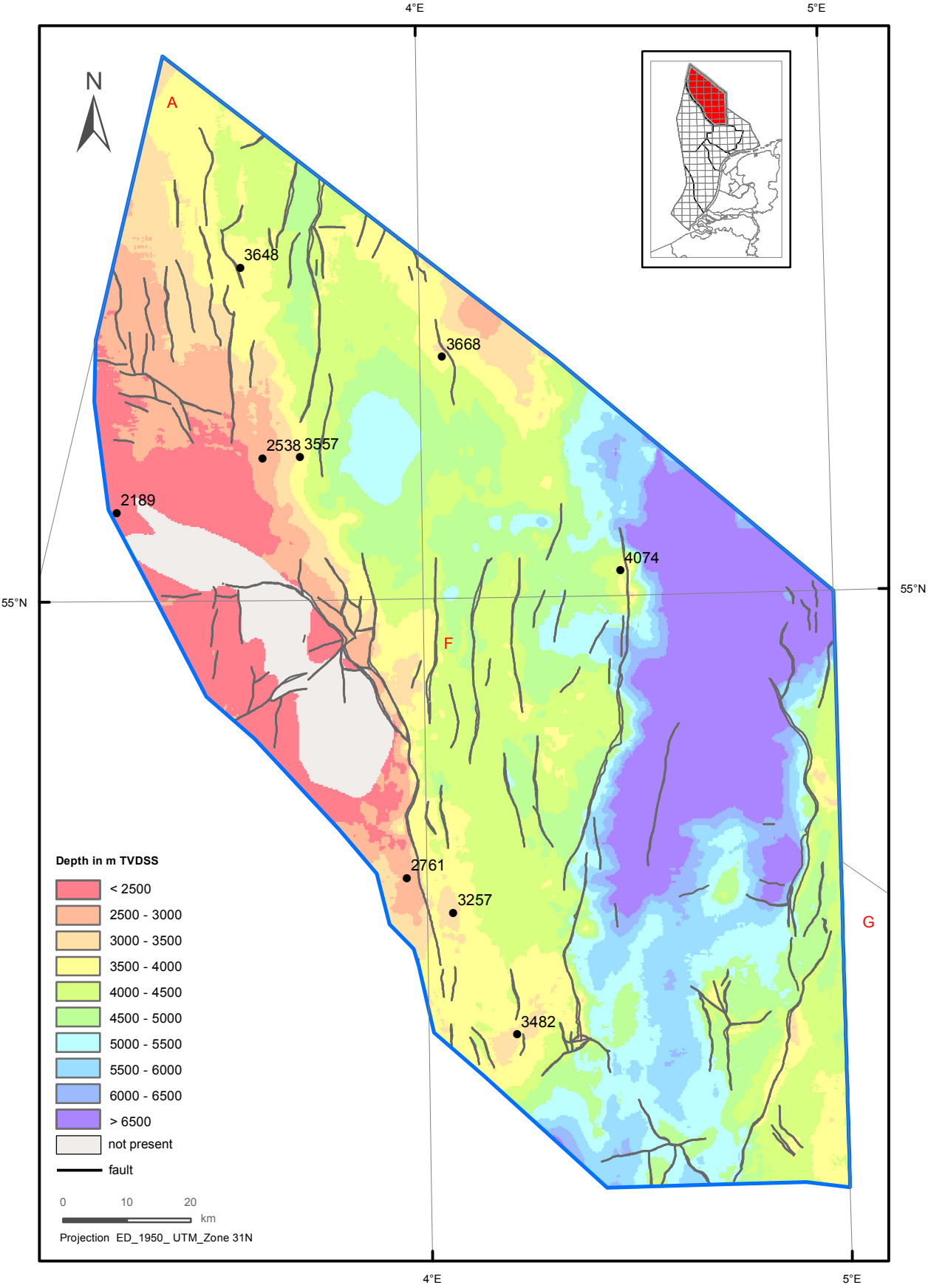
Depth of the base of the Zechstein Group
