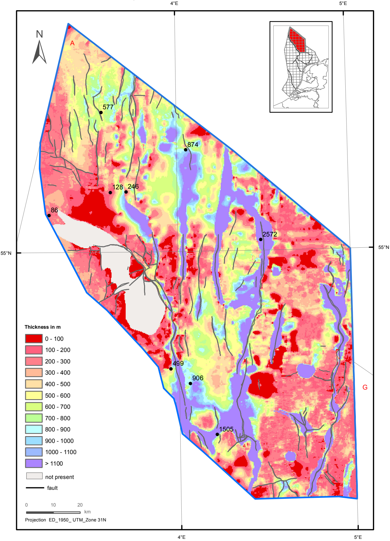
Thickness of the Zechstein Group
